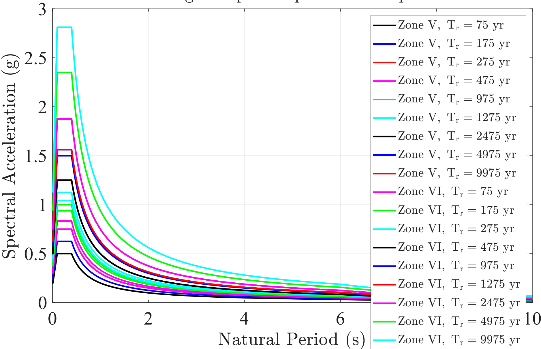
IS Design Response Spectrum Comparison
